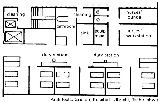
② Intensive care group with 12 beds: St Vinzenzstift Hospital, Hanover
